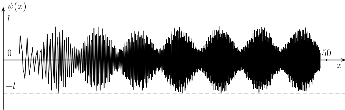
Figure 1: Plot of the function \psi from example 1.
