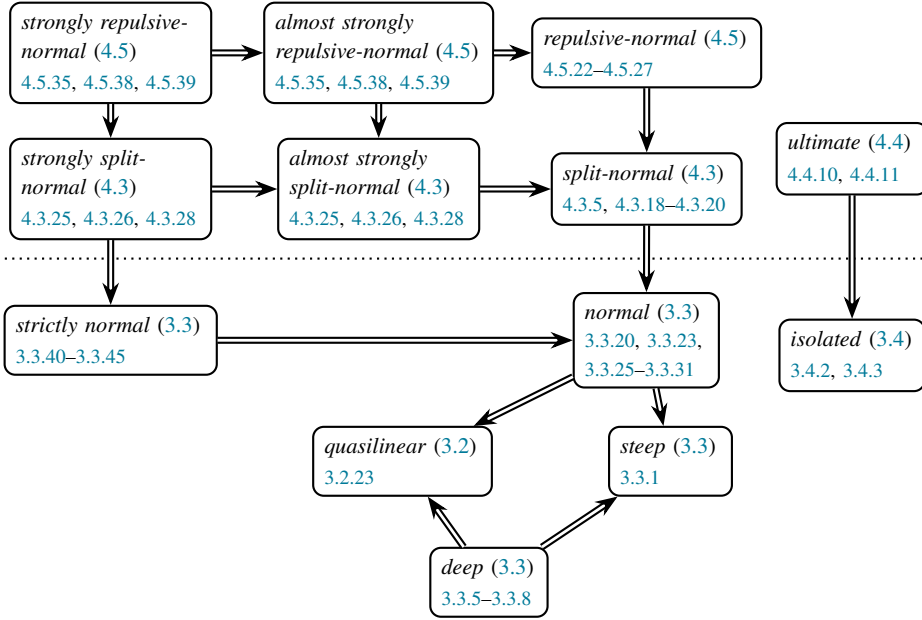
Figure 1. Implications between normality conditions.
